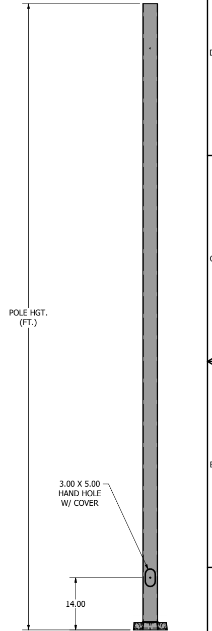
POLE DETAIL
